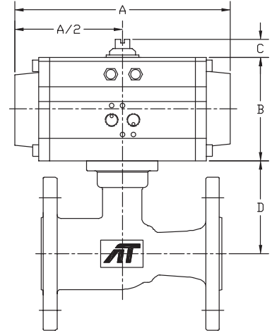
150# Flanged Firesafe tested to API-607
