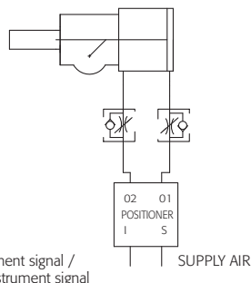
Double acting with flow controls and positioner
