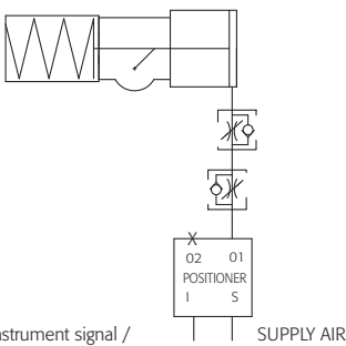
3-15 instrument signal / 4-20 mA instrument signal
