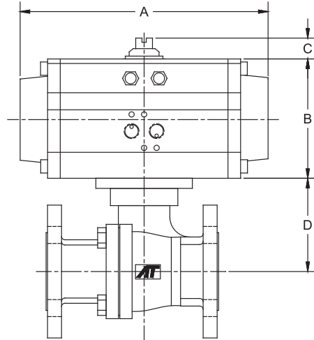
ASME Class 150 Firesafe Tested to API-607 Direct Mount
