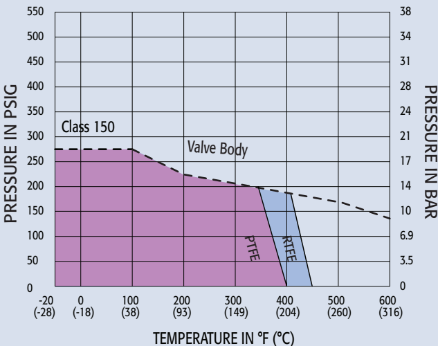
Pressure vs. Temperature Chart
