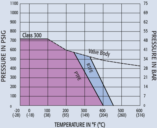
Pressure vs. Temperature Chart for Valves 1/2" to 6"
