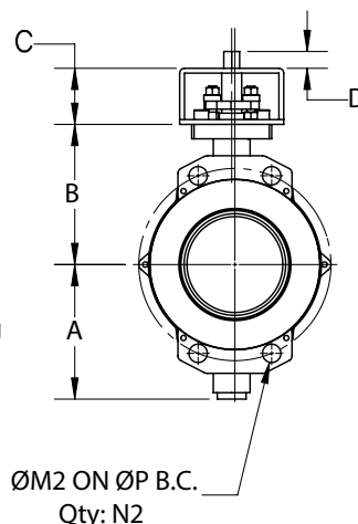
WAFER STYLE BODY
