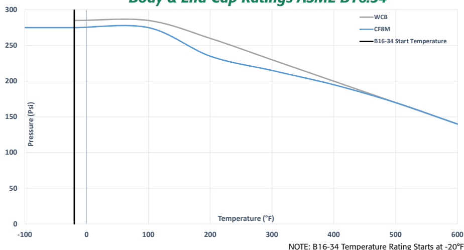
Component Temperature Ratings
