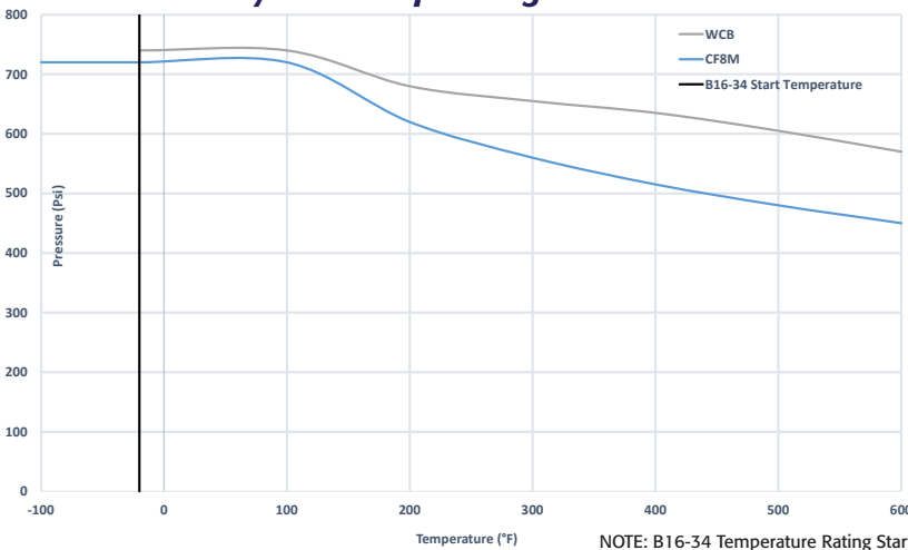
Pressure vs. Temperature - Series FD9-F3 Body & End Cap Ratings ASME B16.34
