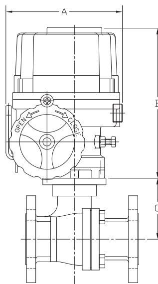
ASME Class 600 Flanged Firesafe Tested to API-607 Direct Mount
