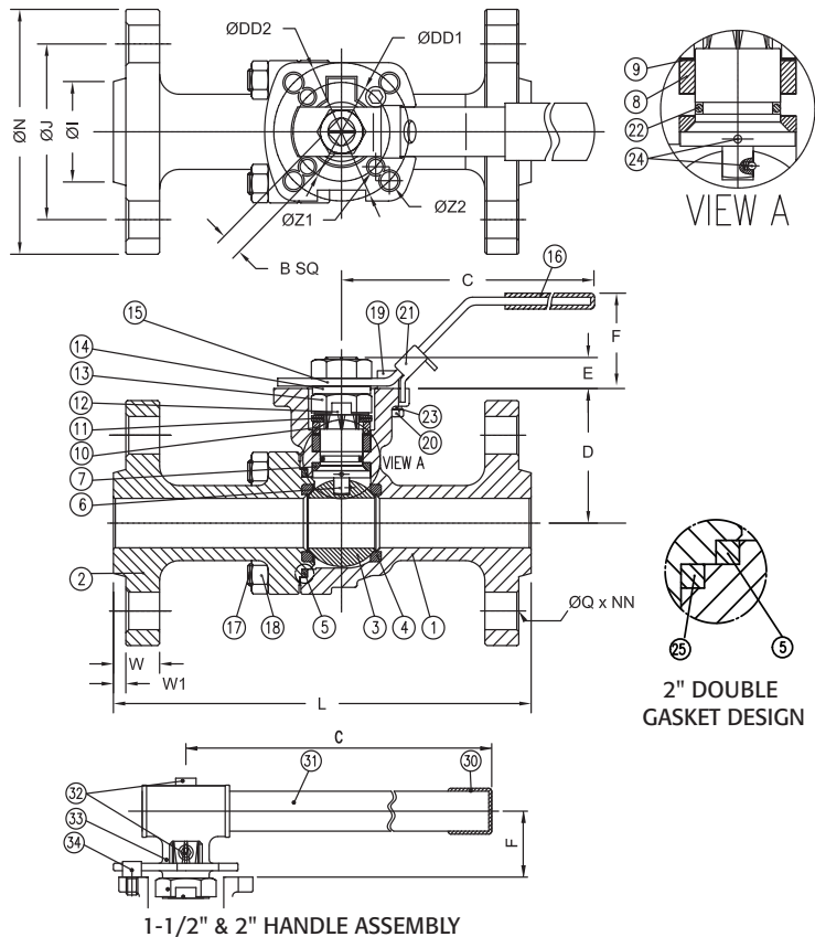
1-1/2" & 2" HANDLE ASSEMBLY
