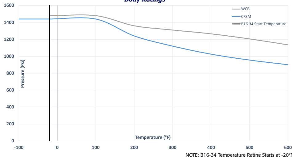
FD9-F6 Component Temperature Ratings
