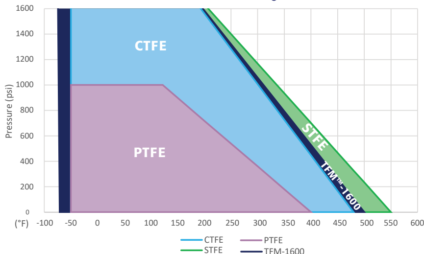
Pressure vs. Temperature - Series D9/FD9-F6 Body Ratings
